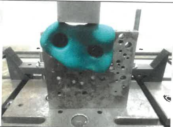
Photo C: Test setup
